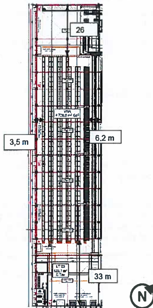
Figure 3 : Plan de racking cellule VNA
